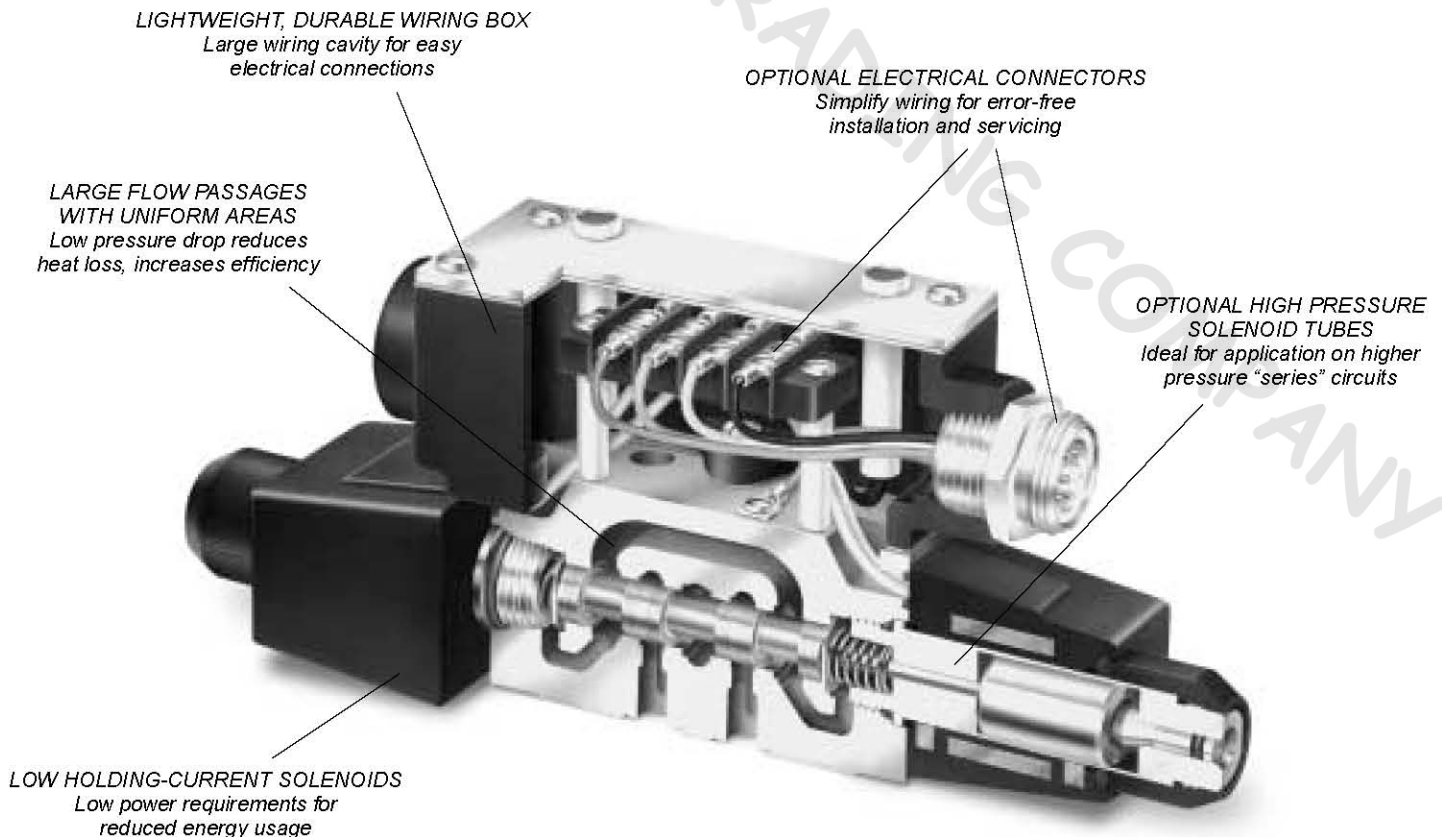
D03 Pattern Directional Control Valve
