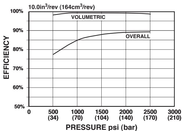
EFFICIENCY @ 1800 rpm
