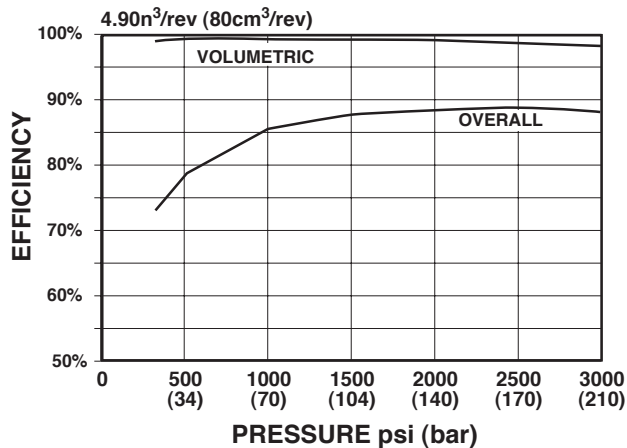
EFFICIENCY @ 1800 rpm
