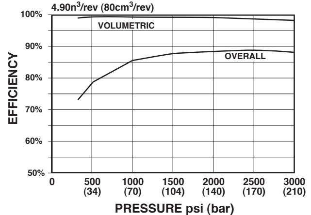
EFFICIENCY @ 1800 rpm
